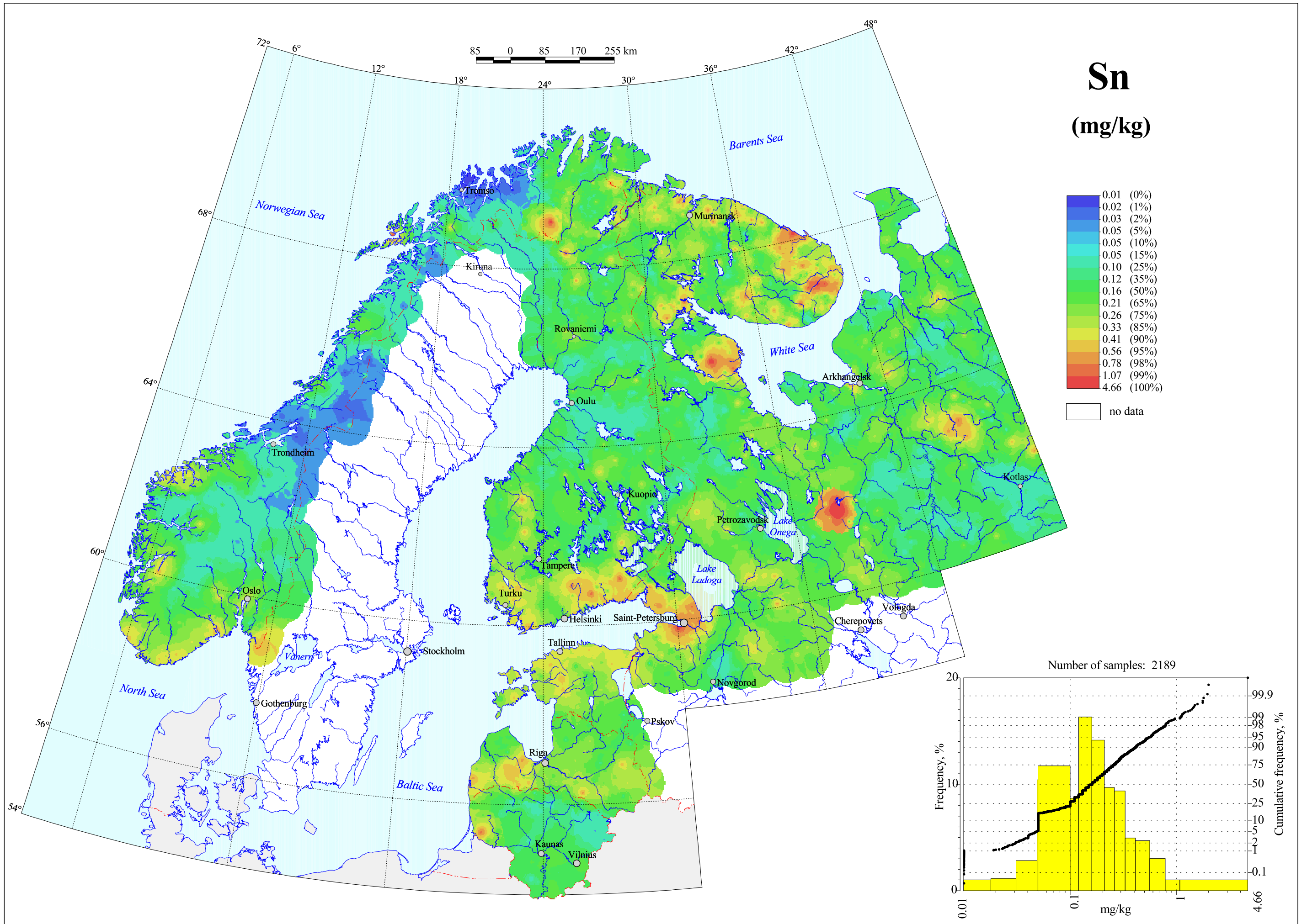
Tin in Terrestrial Moss, Total Content
